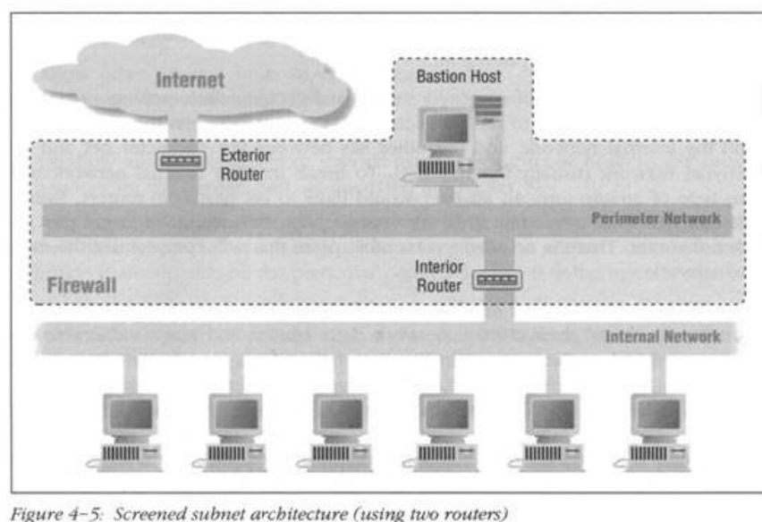
Figure 4-5: Screened subnet architecture (using two routers)
